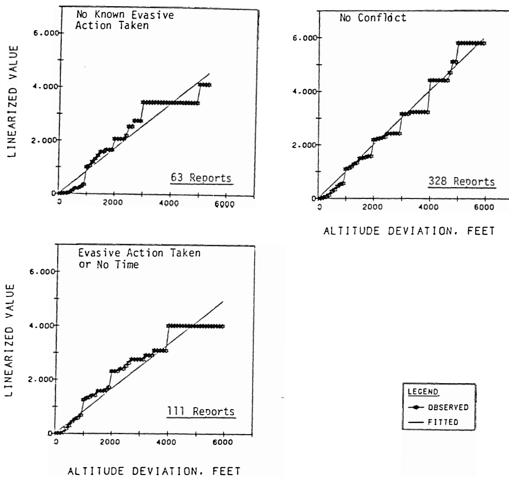
Figure 5d. Deviations Partitioned By Conflict and Evasive Response
