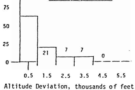
FIGURE B-1. OBSERVED DISTRIBUTIONS OF ALTITUDE DEVIATIONS BY FLIGHT PATTERN GROUPS
