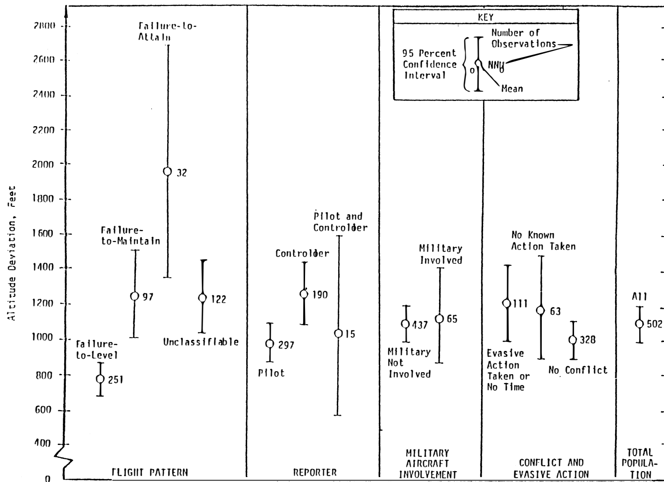
FIGURE 6. MEANS OF EXPONENTIAL DISTRIBUTION OF SUBGROUPS
