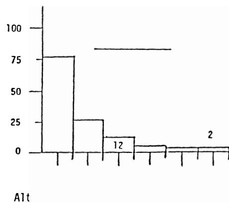
FIGURE B-1. OBSERVED DISTRIBUTIONS OF ALTITUDE DEVIATIONS BY FLIGHT PATTERN GROUPS
