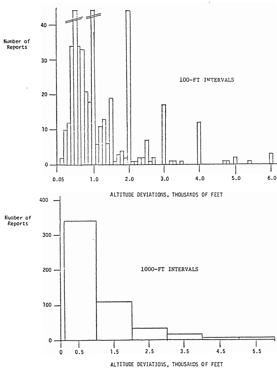
FIGURE A-1. ALTERNATIVE HISTOGRAMS OF REPORTED ALTITUDE DEVIATIONS
